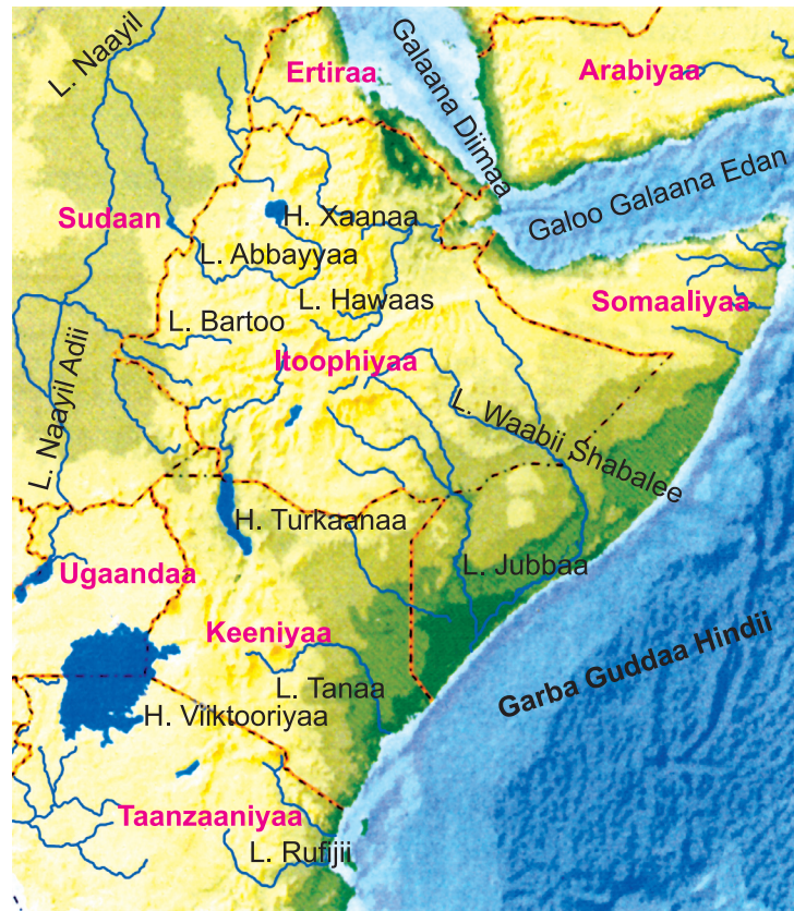
Fakkii 2.4. Qabeenya bishaanii naannoo Baha Afrikaa
