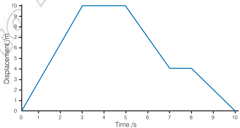
Figure 2.9 Distance–time and displacement–time graphs for the same journey.
