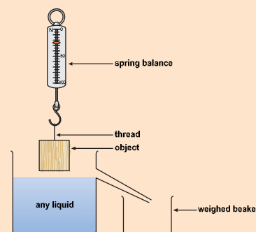
Figure 6.51 Testing Archimedes's principle
