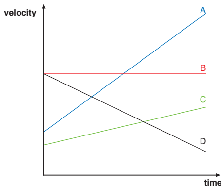
Figure 2.31 Velocity–time graphs for four cars.
