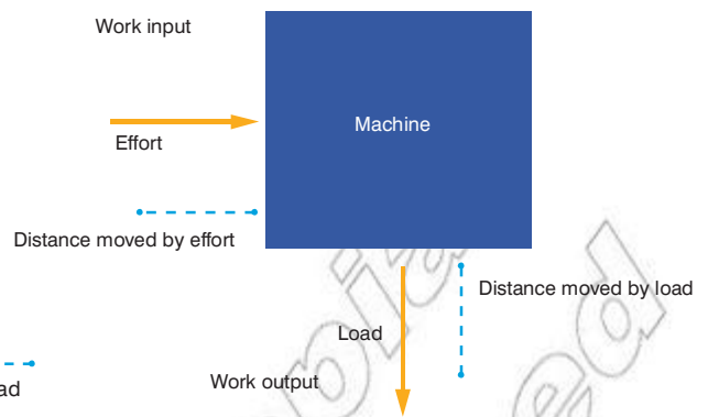
Figure 5.7 A schematic of a direction changer. Notice the load is moved in a different direction to the effort.
