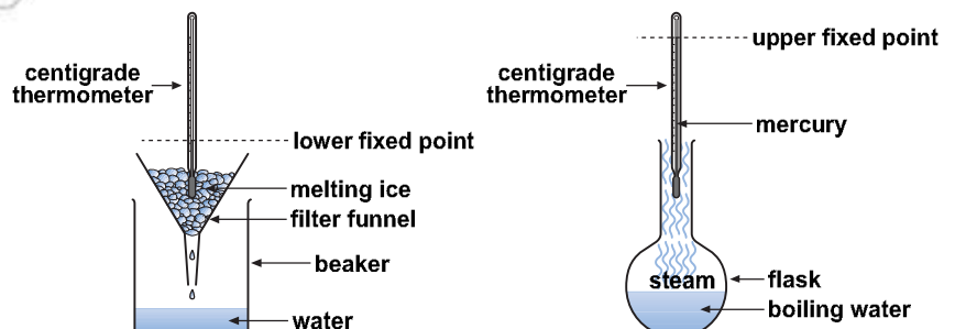
Figure 7.31 Calibrating a thermometer
