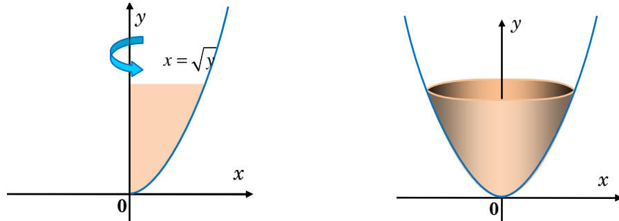
a The region to rotated about the y -axis b The solid of revolution Figure 5.38
